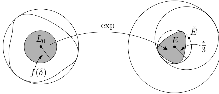
Figure 2: Everything within an f(\delta) -ball around L_0 is mapped into an \varepsilon/3 -ball around E , which itself is contained within a 2\varepsilon/3 -ball around \tilde{E} . (See also Fig. 1.)
