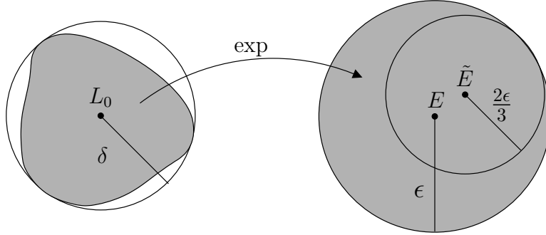
Figure 1: The pre-image of an \varepsilon -ball around E = e^{L_0} is contained within a \delta -ball around L_0 . If \tilde{E} is within \varepsilon/3 of E , then everything within a 2\varepsilon/3 -ball around \tilde{E} is within the \varepsilon -ball around E .
